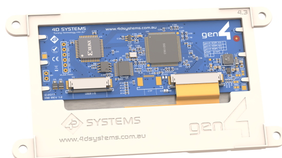
Resistive Touch Display configuration shown.
