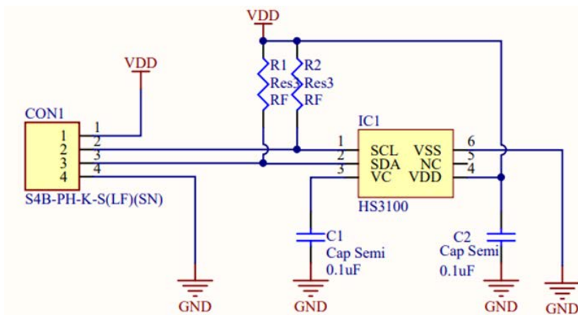
Figure 14. HS300x-MC1 Application Circuit
