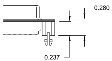
05 ..... 0.237" (SOLDER SIDE)
