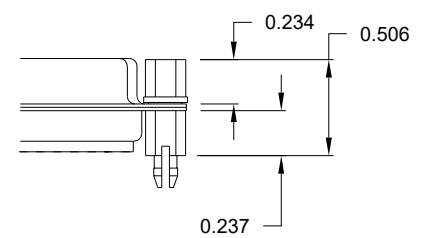
91 ..... 0.237" (SOLDER SIDE)
