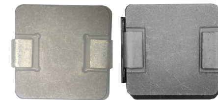
Scratches: acceptable Scratches may be seen on the surface of the inductor body. Scratches are an acceptable surface irregularity.
