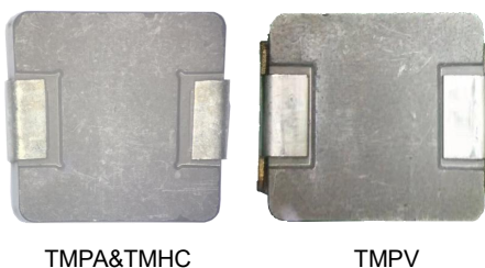
Yellowing : PAD yellowing ratio less than 20% is OK
