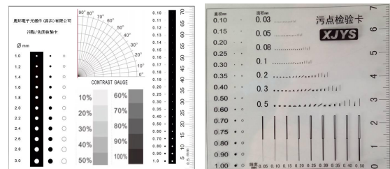
Blackening:PAD black/ brightness ratio less than 20% is OK
