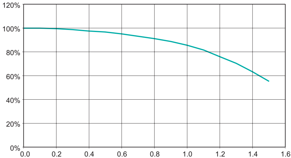
Inductance vs. Current Characteristics
