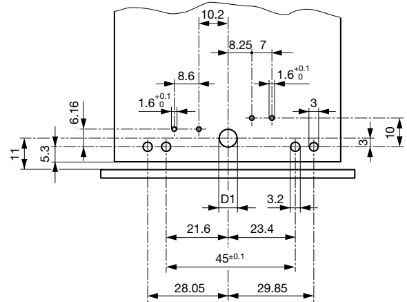
Drilling Diagram / CMF1 and CMF2
