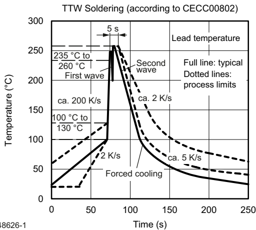
Fig. 27 - Wave Soldering Double Wave Profile According to J-STD-020 for DIP Devices
