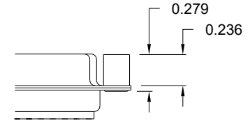
03 ..... 0.236" (MATING SIDE)
