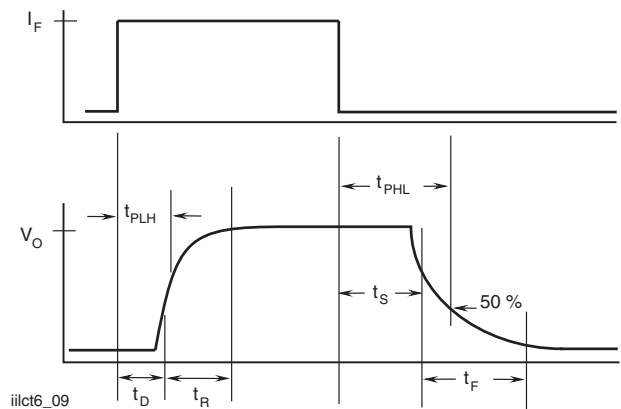
Fig. 9 - Switching Timing
