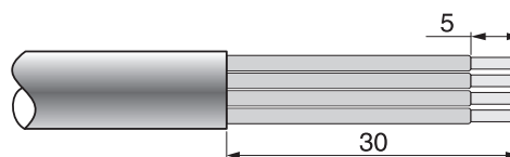
Figure 2-20 Preparing the cable
