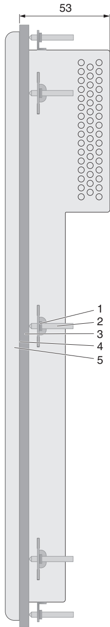
Figure 2-19 Side view, mounting depth (dimensions in mm)
