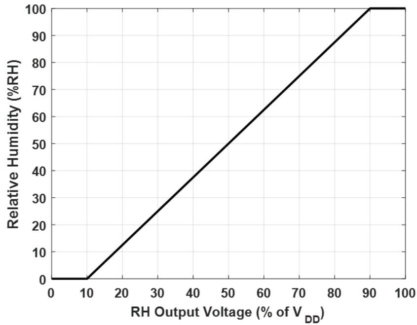
Figure 9. Relative Humidity vs. VRH Output Analog Voltage
