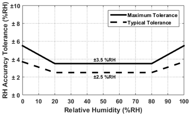
Figure 4. HS41x3 RH Accuracy Tolerance at 25°C
