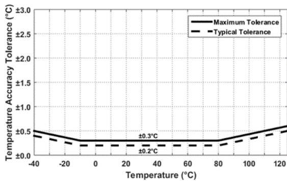
Figure 6. HS41x1 Temperature Sensor Accuracy Tolerance
