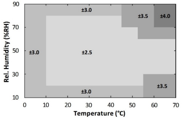
Figure 5. HS41x3 RH Accuracy over Temperature
