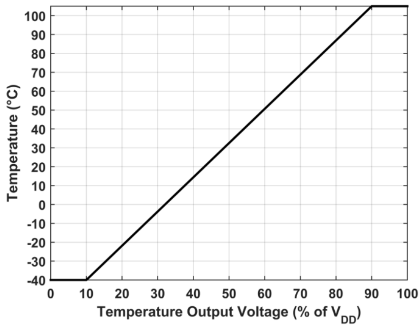
Figure 10. Temperature vs. VT Output Analog Voltage
