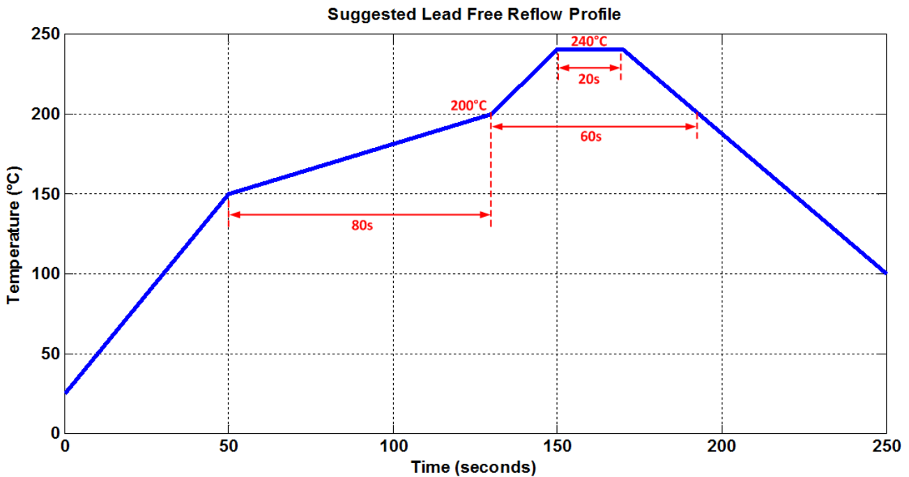
Figure 11. Recommended Soldering Profile
