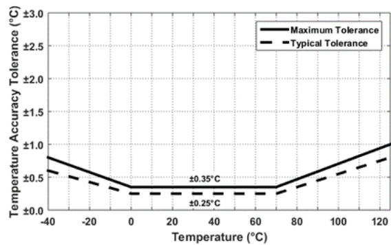
Figure 7. HS41x3 Temperature Sensor Accuracy Tolerance
