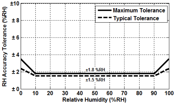
Figure 2. HS41x1 RH Accuracy Tolerance at 25°C
