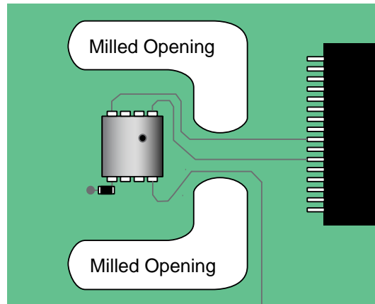
Figure 12. Milled PCB Openings for Thermal Isolation
