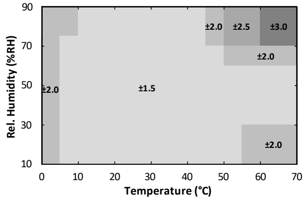
Figure 3. HS41x1 RH Accuracy over Temperature
