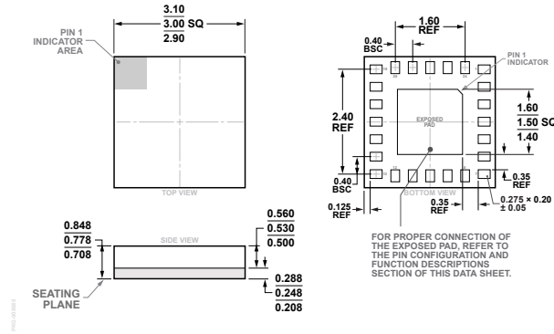
Figure 28. 24-Terminal Land Grid Array [LGA] 3 mm x 3 mm Body and 0.778 mm Package Height (CC-24-14) Dimensions shown in millimeters
