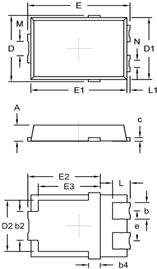
TO-277A (SMPC4.6U)
