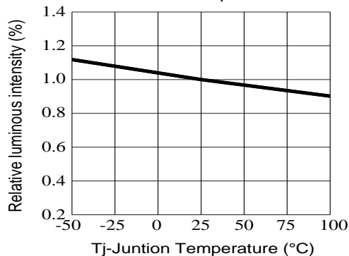
Fig.3-Relative Luminous Intensity vs. Junction Temperature
