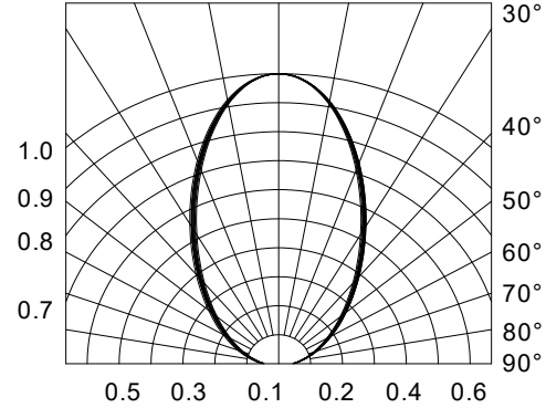
Fig.6-Radiation Diagram Ta=25°C
