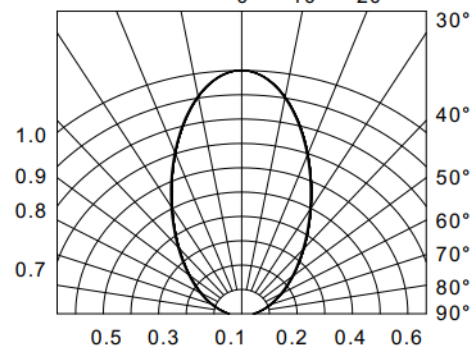
Fig.6-Radiation Diagram
