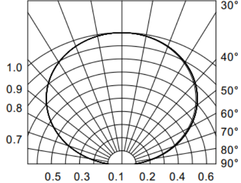
Fig.6-Radiation Diagram Ta=25°C
