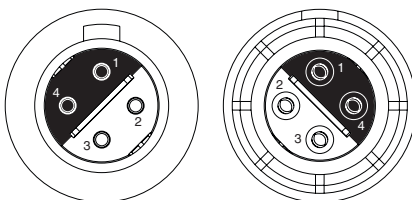
PIN CONTACT MATING FACE
