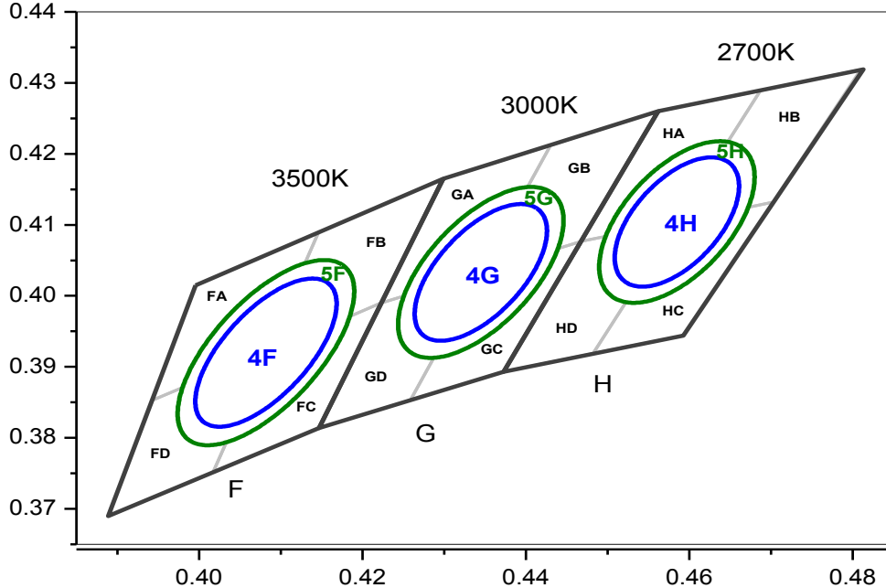
CIE Chromaticity Diagram, T_j=85^\circ\text{C} , I_f=700\text{mA}
