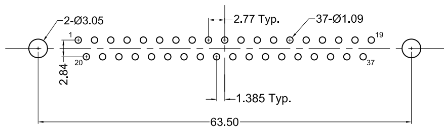
Recommended PCB Layout (Top View)
