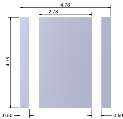
3-V and 6-V PCB Footprint Depending on Vf Class (Thermal pad is electrically isolated)
