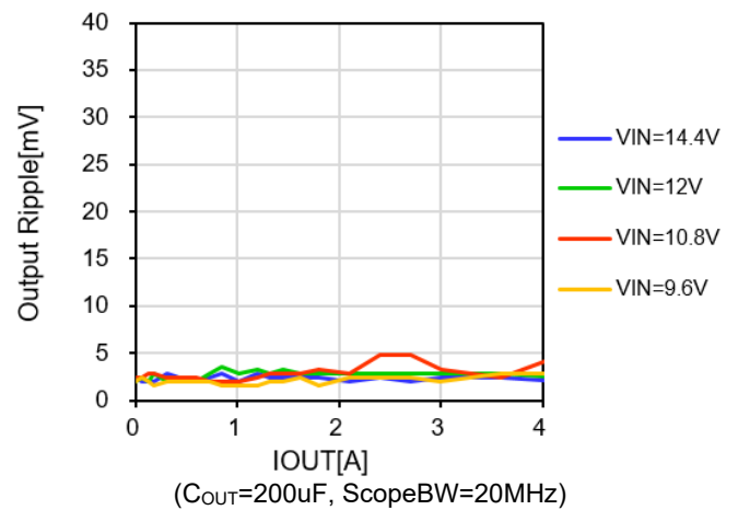
Figure 14. Output Ripple and Noise (C OUT =200uF, ScopeBW=20MHz)
