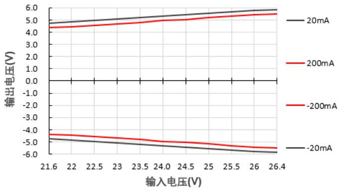
输出电压Vs输入电压@A2405S-2WR3
