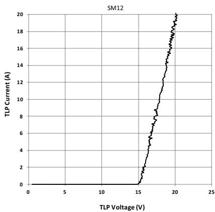
SM12 Transmission Line Pulsing(TLP) Plot
