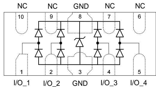
4-Line Protection
