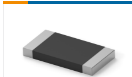
TE 产品编号4-2176422-0 TLRP 2512 3.0W R090 1% 25PPM 4K RL
