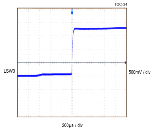
LDO3 Load Switch Mode Start up
