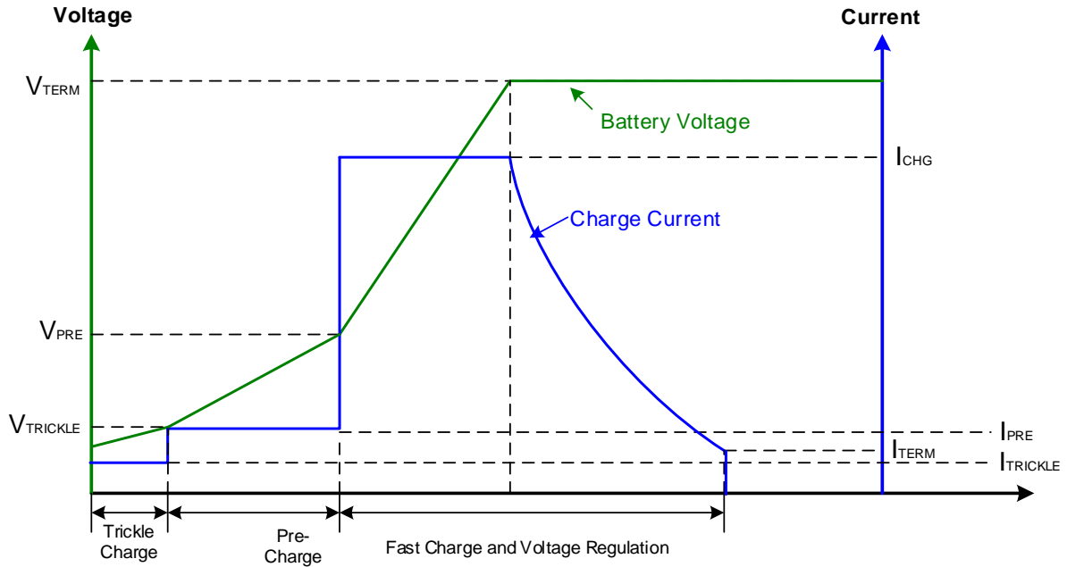
Figure 3: APLC Charging Profile
