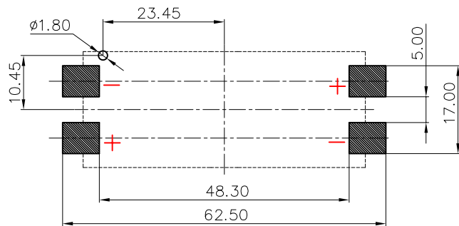
PCB Layout Diagram Top View
