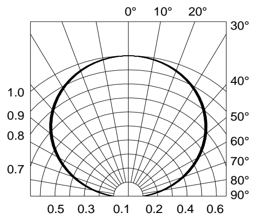
Fig.6-Radiation Diagram Ta=25°C
