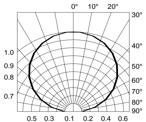
Fig.6-Radiation Diagram T_a=25^\circ\text{C}
