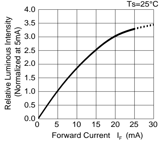
Fig.2-Relative Luminous Intensity vs. Forward Current T_s=25^\circ\text{C}
