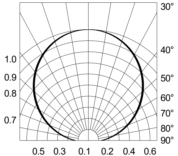
Fig.6-Radiation Diagram Ta=25°C
