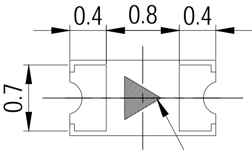
Cathode Mark
