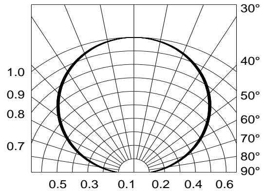
Fig.6-Radiation Diagram
