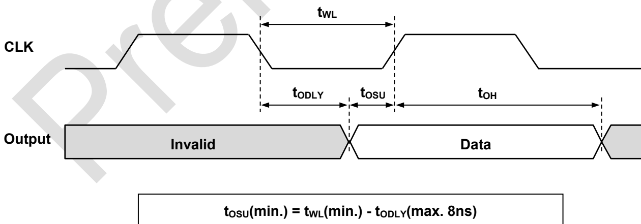
Figure 2 Output timing
