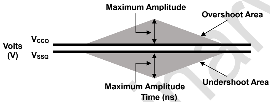
Figure 4 Overshoot / Undershoot definition
