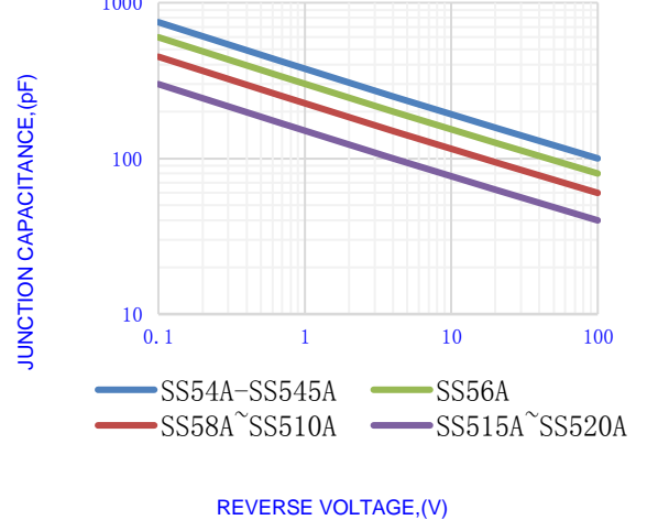
Fig.4-TYPICAL JUNCTION CAPACITANCE
