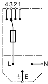
with internal connections Voltage Selector 4-positions, 1-pole
