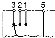
Voltage Selector 3 pos. 2-pole
