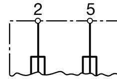
without voltage selector 2-pole
