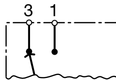
Voltage Selector 2 pos. 1-pole
