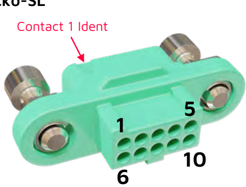
Female Crimp Housing
