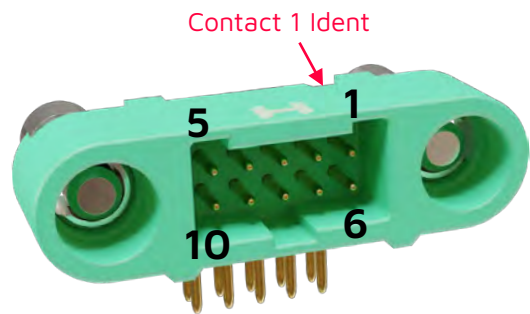
Male PCB mounted
