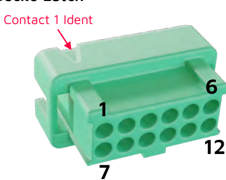
Female Crimp Housing
