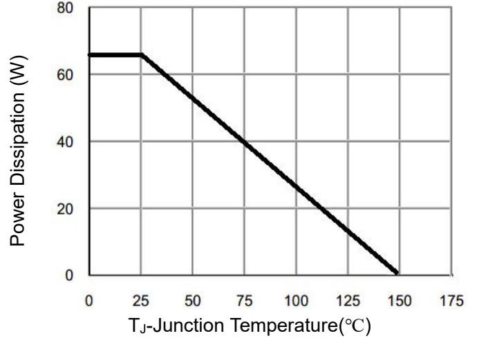
Figure 9 Power De-rating
