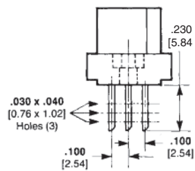
Solder Eyelet Contact
