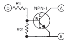
SCHEMATIC DIAGRAM
