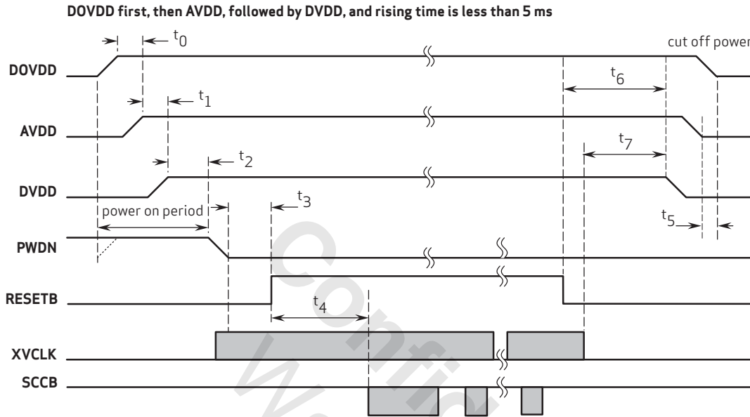
figure 2-5 power up timing with external DVDD source
