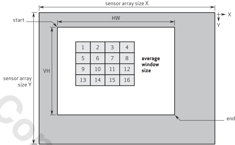
figure 4-6 average-based window definition
