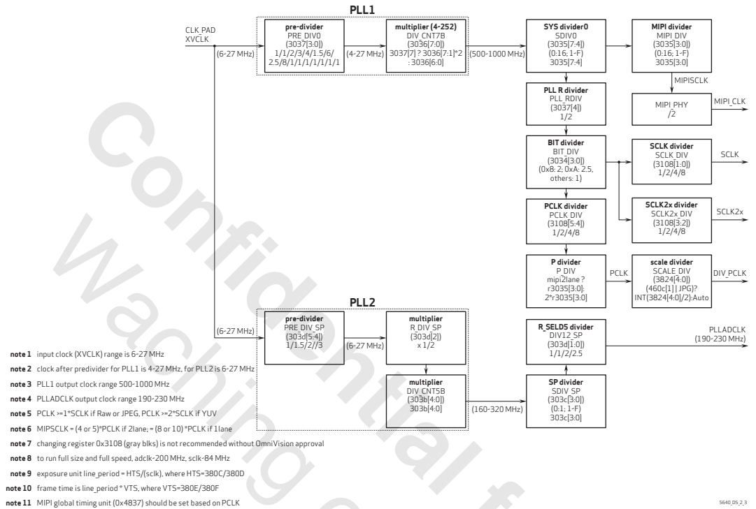
figure 2-3 PLL diagram
