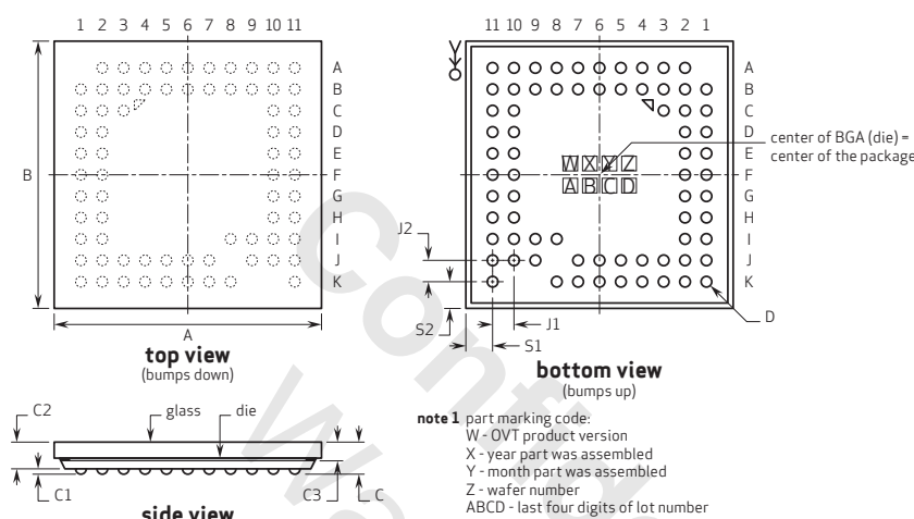
figure 9-1 package specifications
