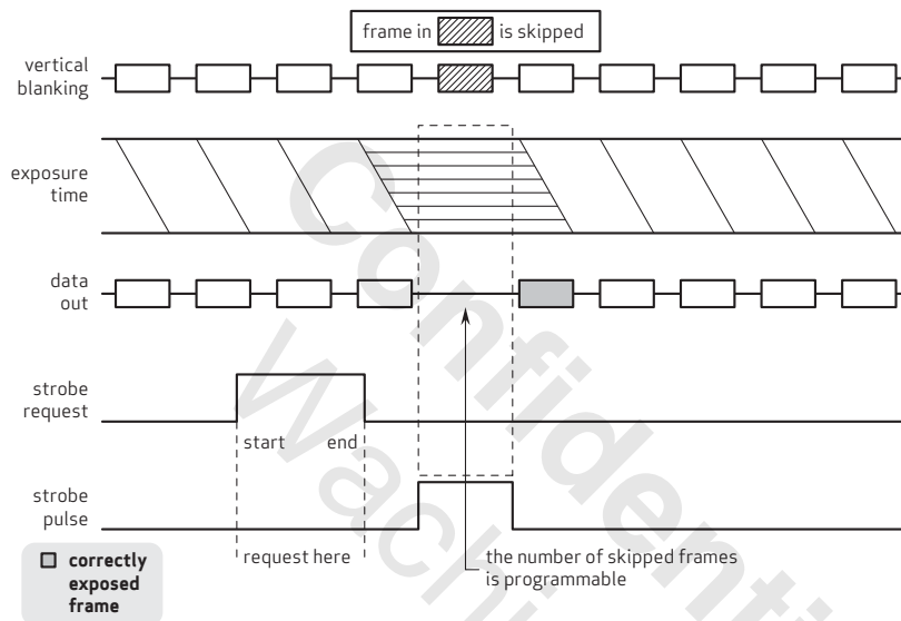
figure 4-8 LED 1 & 2 mode - one pulse output
