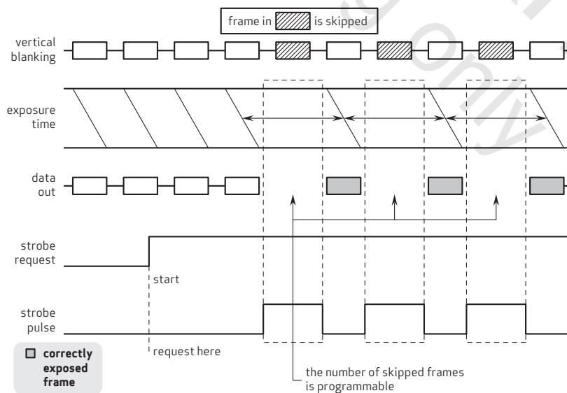
figure 4-9 LED 1 & 2 mode - multiple pulse output
