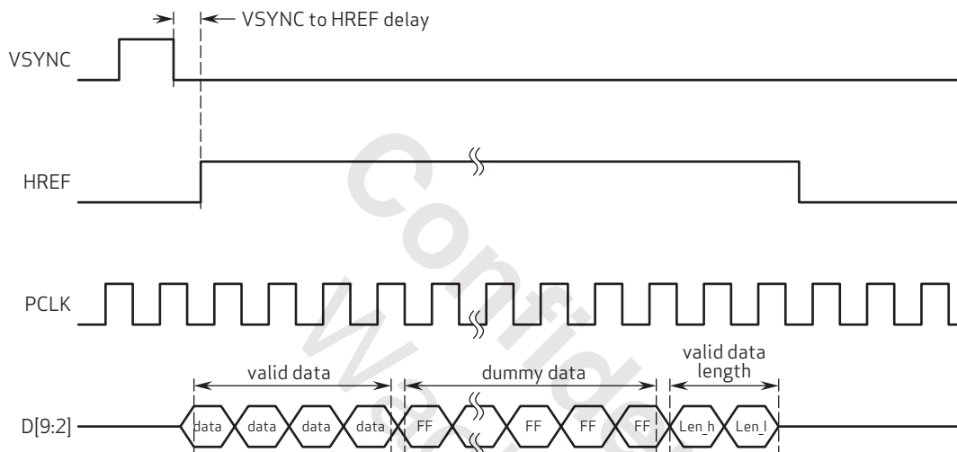
figure 6-5 compression mode 5 timing
