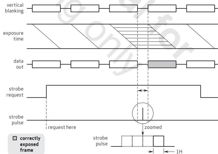
figure 4-7 xenon flash mode
