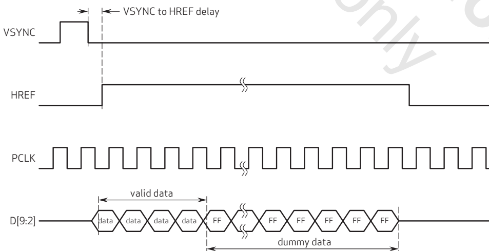
figure 6-6 compression mode 6 timing
