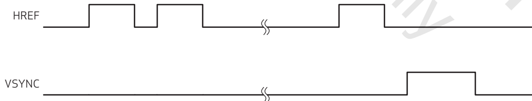
figure 6-2 compression mode 2 timing
