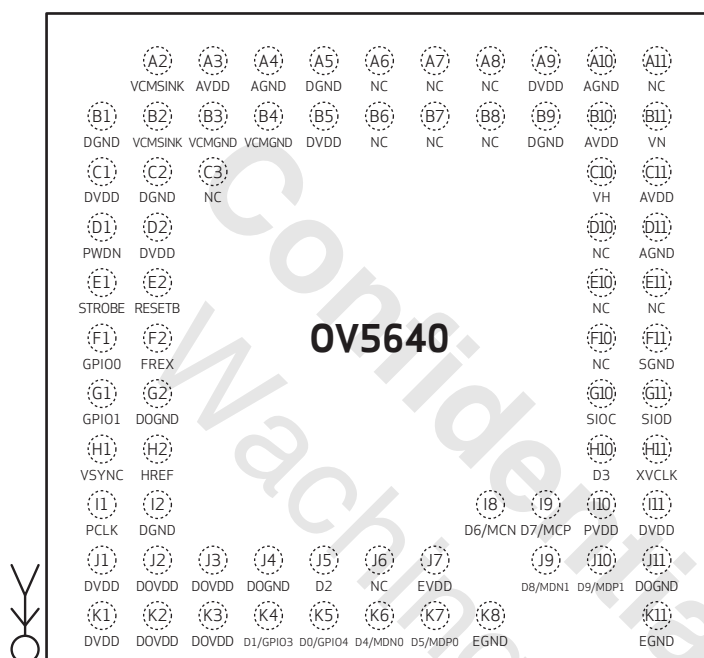
figure 1-1 pin diagram
