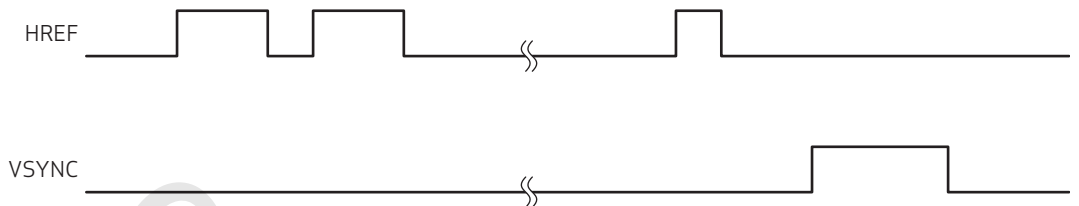
figure 6-3 compression mode 3 timing
