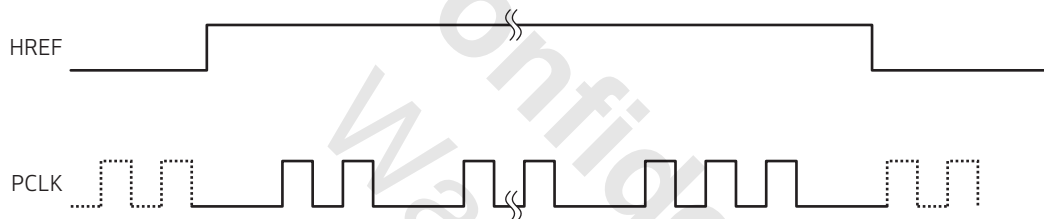
figure 6-1 compression mode 1 timing
