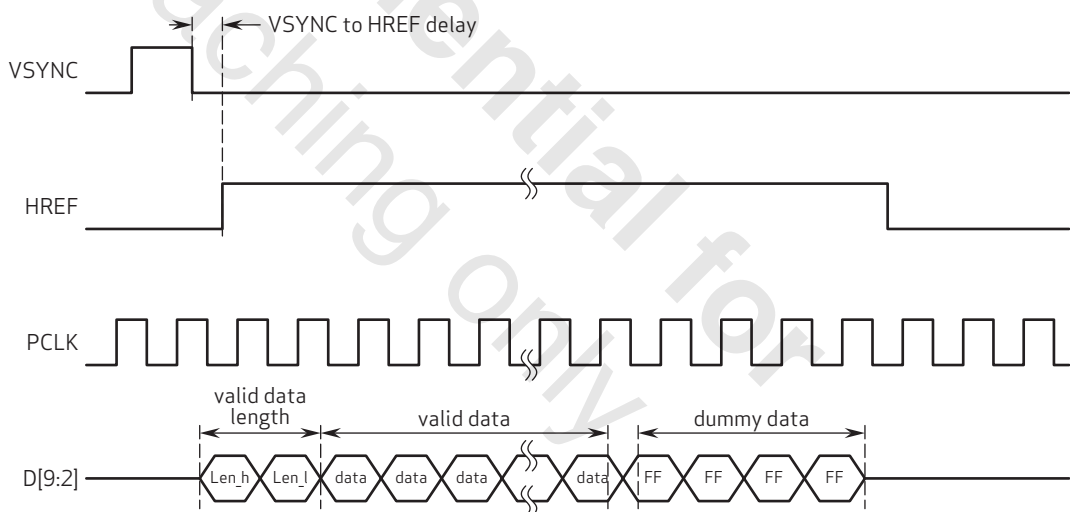
figure 6-4 compression mode 4 timing
