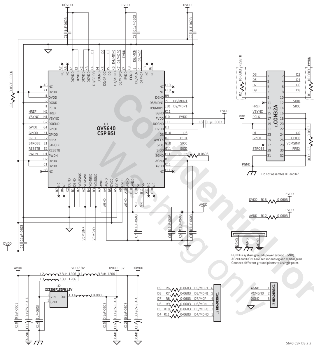
figure 2-2 reference design schematic
