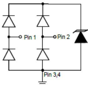
2-Line Protection
