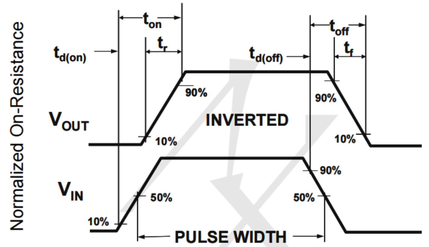
Figure 2: Switching Waveforms
