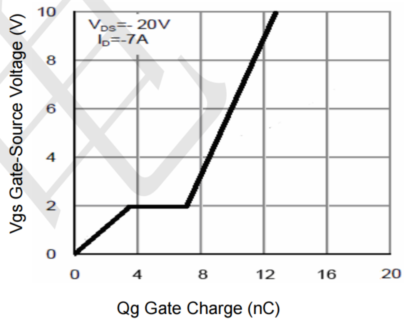
Figure 5 Gate Charge
