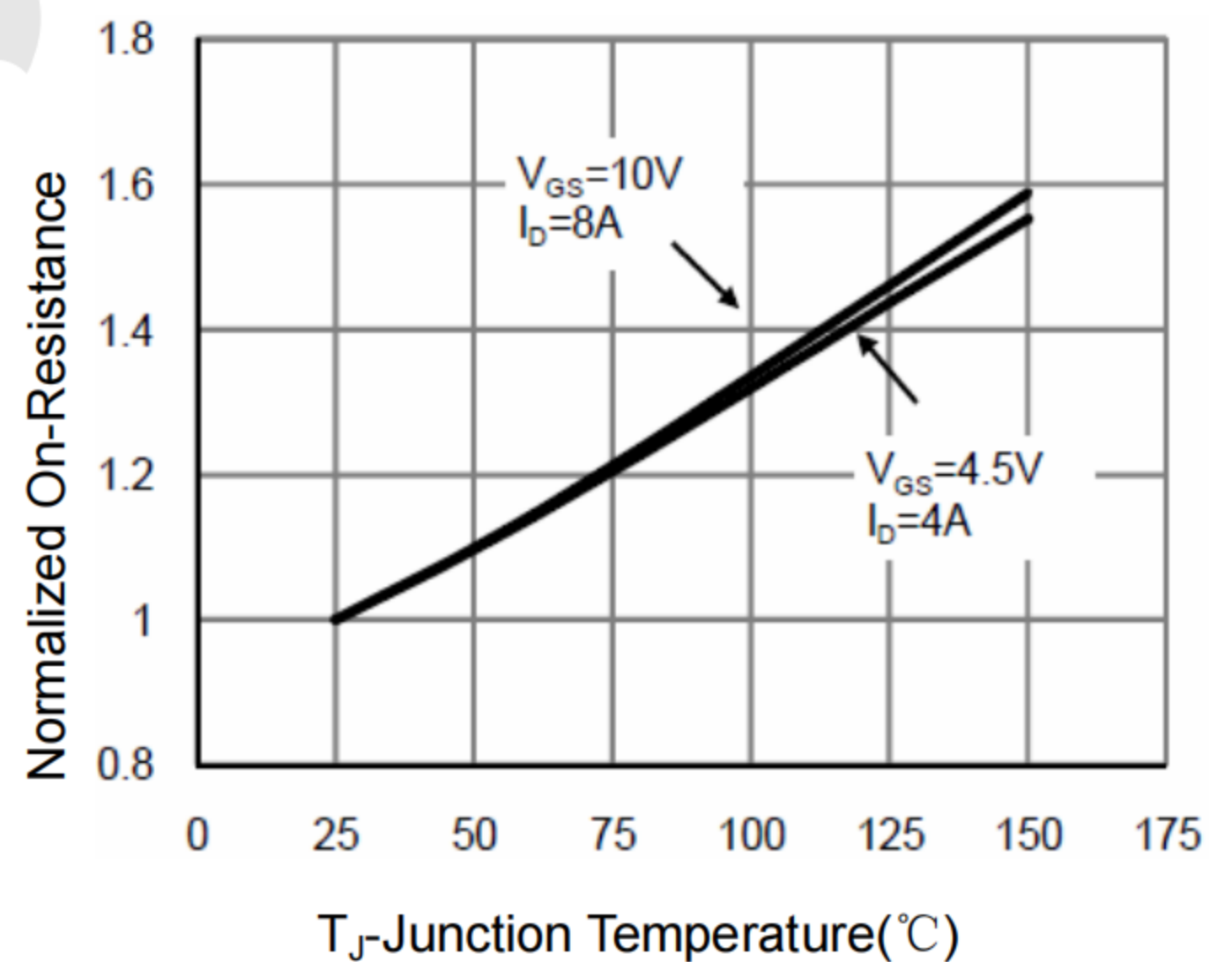
Figure 6 Drain-Source On-Resistance
