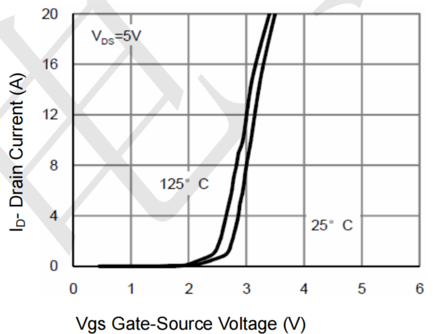
Figure 4 Transfer Characteristics
