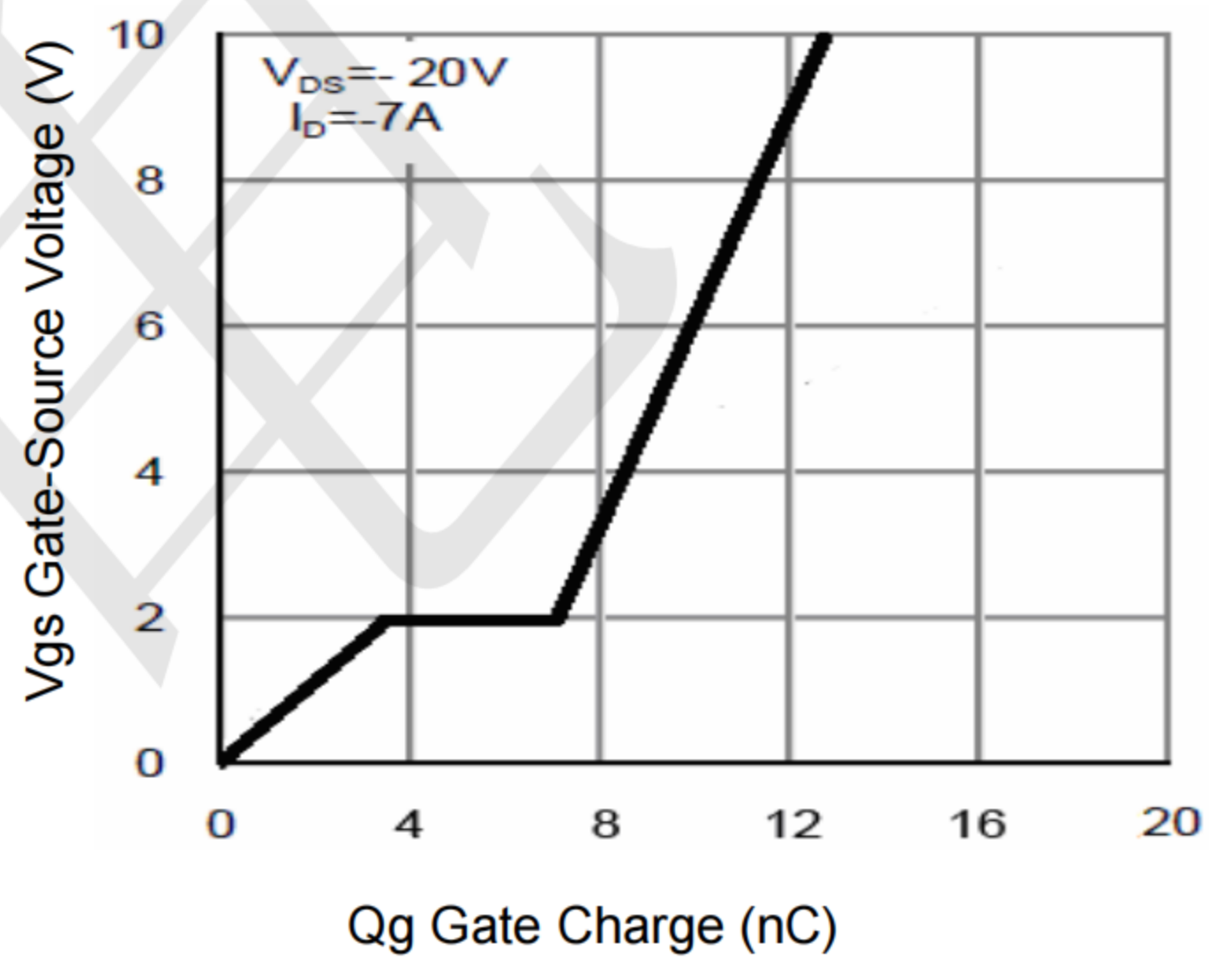
Figure 5 Gate Charge
