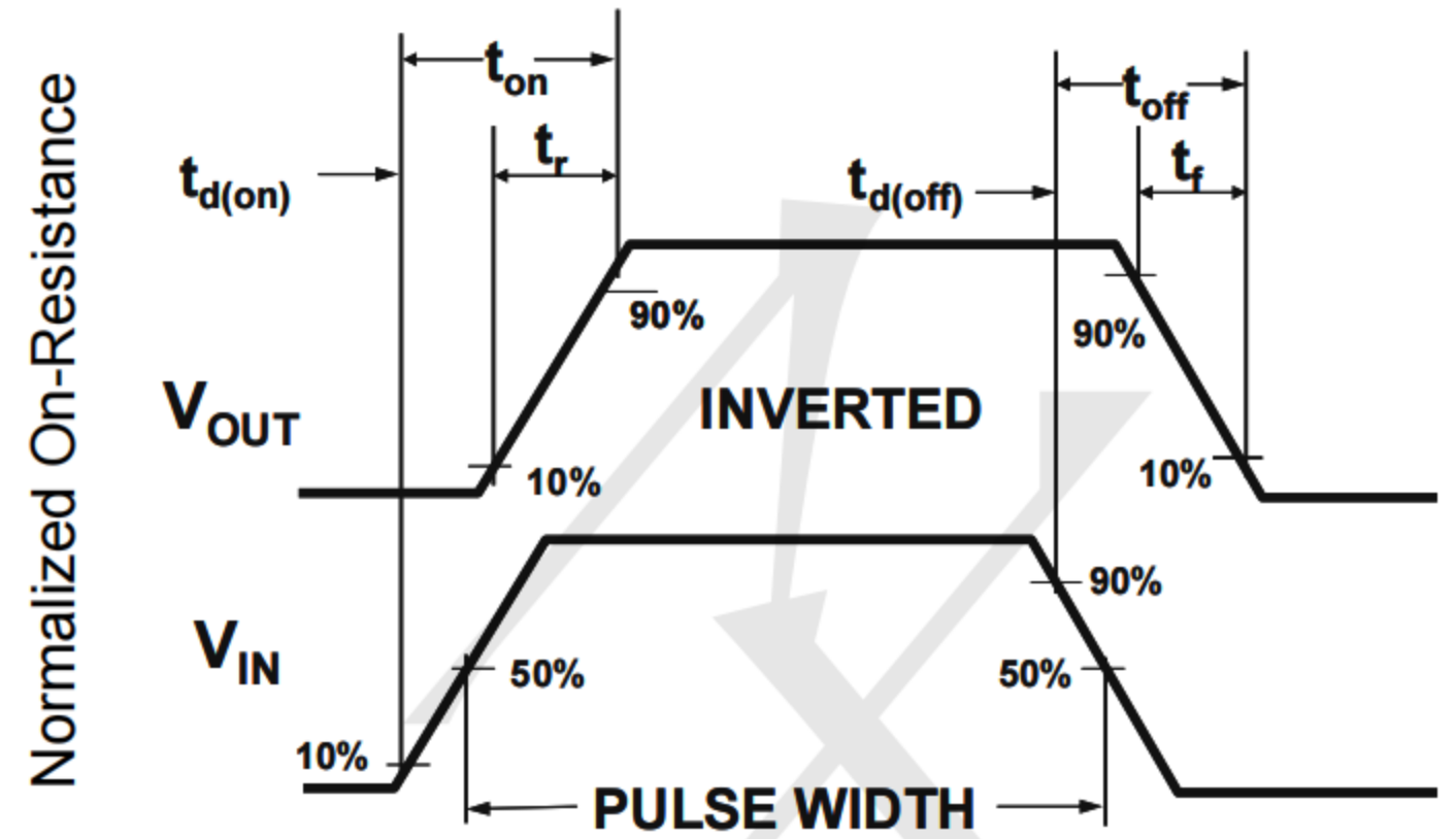
Figure 2: Switching Waveforms
