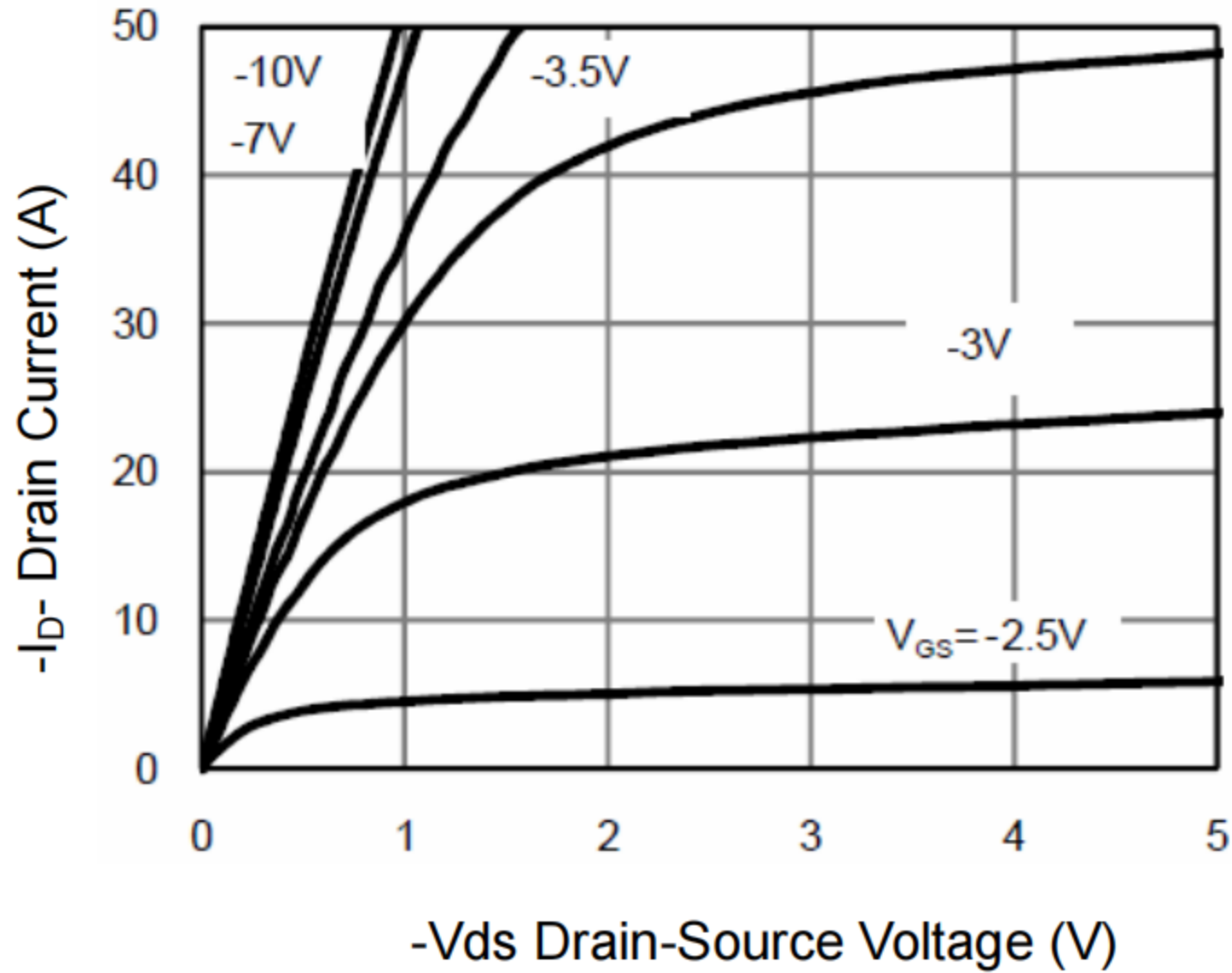
Figure 1 Output Characteristics
