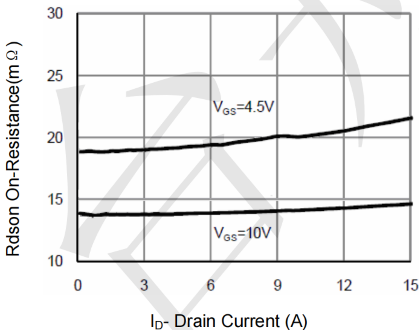
Figure 5 Drain-Source On-Resistance
