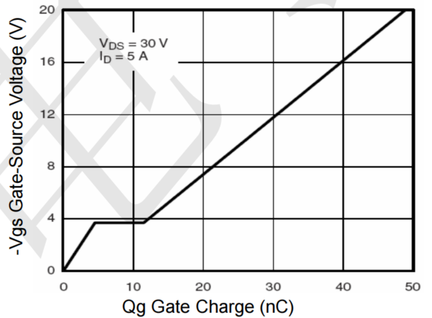
Figure 5 Gate Charge
