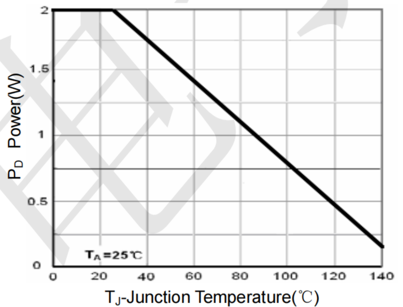
Figure 10 Power Dissipation
