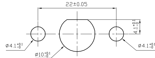
PANEL CUTOUT
