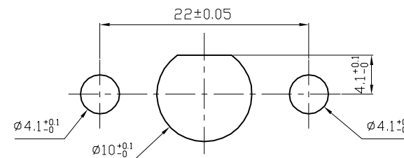
PANEL CUTOUT
