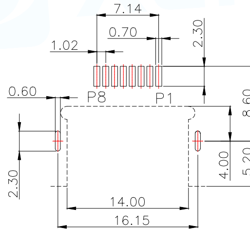
PCB LAYOUT
