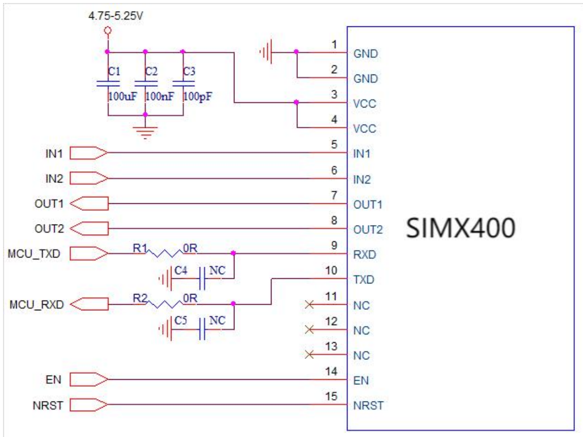
Simplified Reference Circuit
