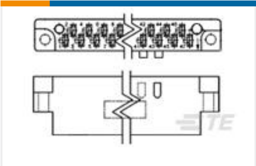
TE Part #3-582151-5 41 AMP BLADE RCPT HSG
