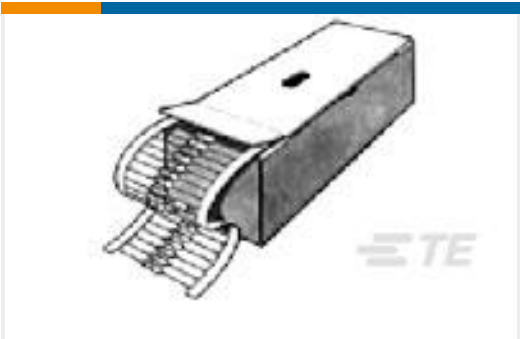
TE Part #1-2176084-2 EP 7W (S) 680R 5%
