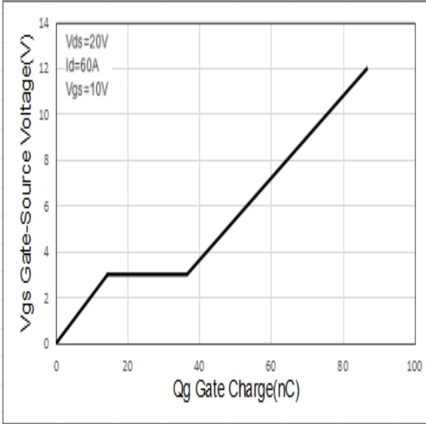
Fig 4. Gate Charge
