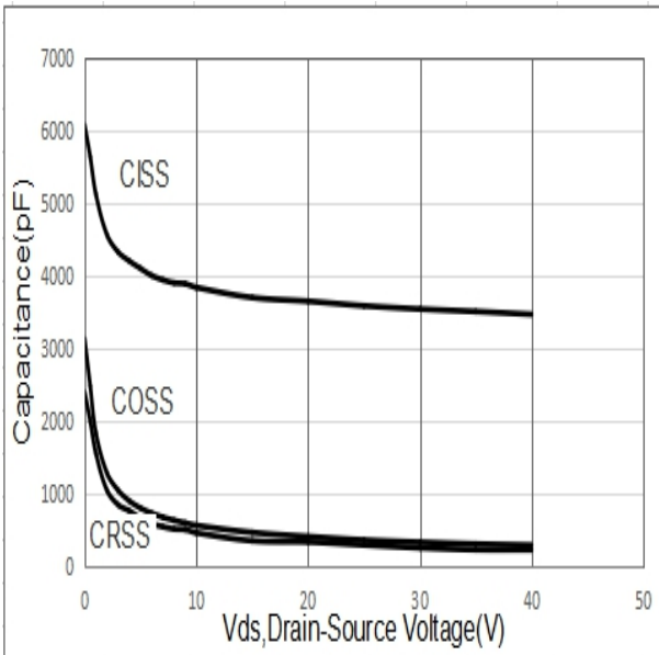
Figure 6. Capacitance Characteristics
